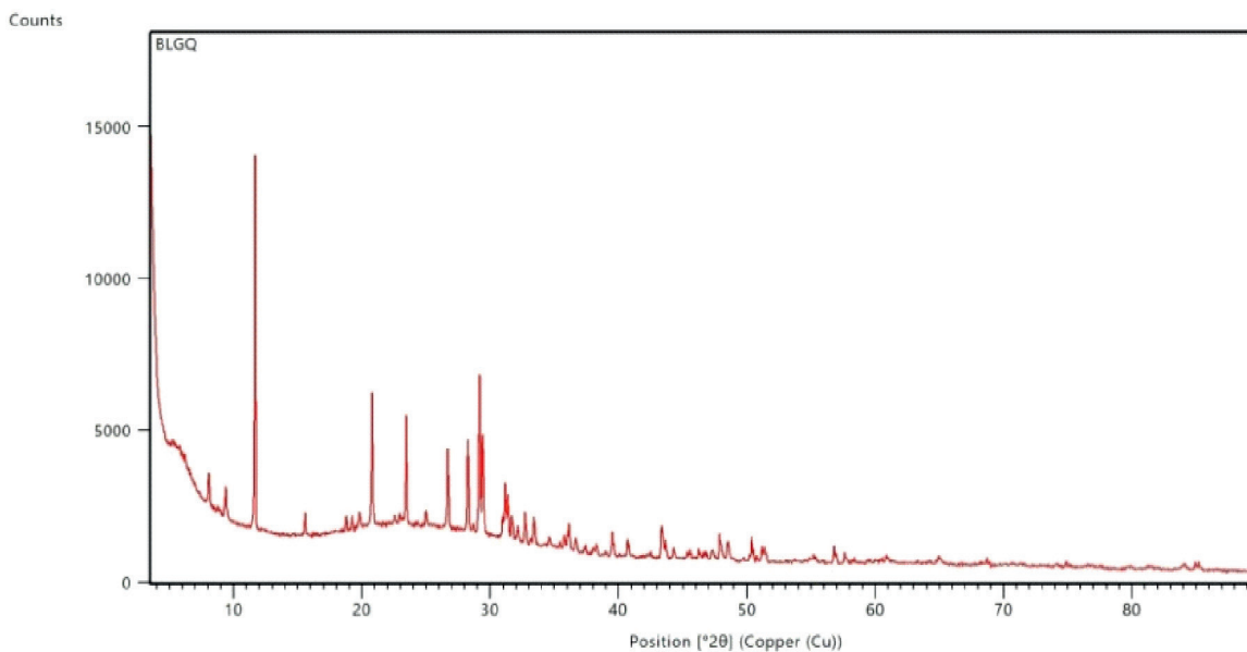
Fig. 9: Representative XRD of Baolagotrench (BLG ES) Baolagog exposed section
